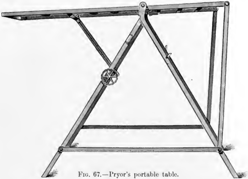
FIG. 67.—Pryor's portable table.
